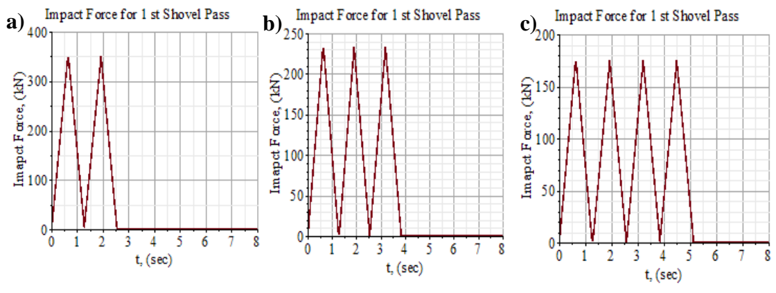
Figure 6.7. Impact Force Plotting for Experiment No. 6 with H_t = 5.0 m a) M = 1 b) M = 2 c) M = 3
