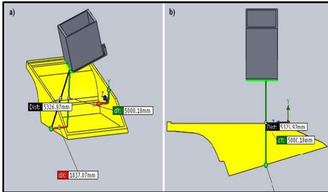
Figure 5.10. Truck Body and Shovel Dipper CAD Assembly for H_t = 5.00\text{ m} (5000 mm): a) Isometric View b) Side View
