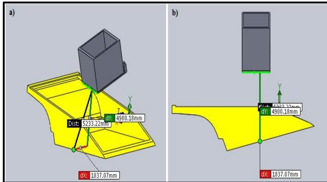
Figure 5.11. Truck Body and Shovel Dipper CAD Assembly for H_t = 4.90\text{ m} (4900 mm): a) Isometric View b) Side View
