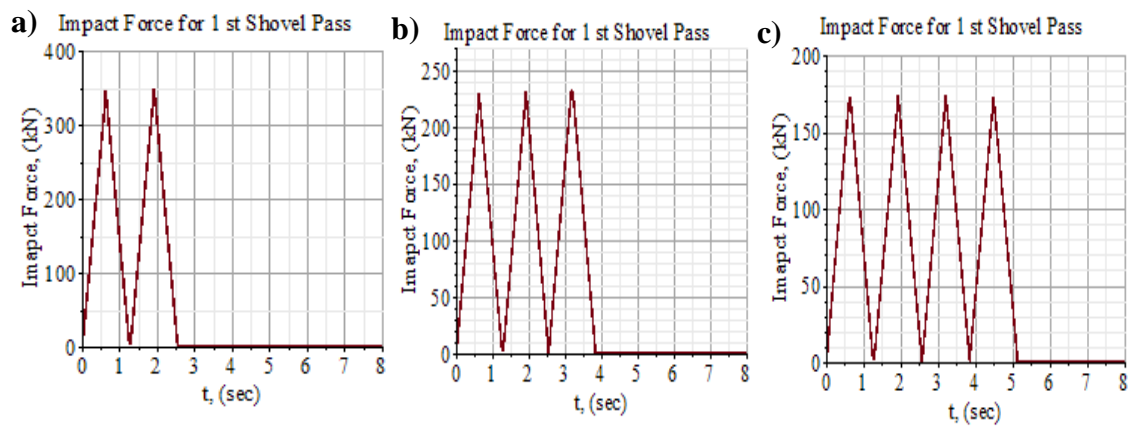
Figure 6.8. Impact Force Plotting for Experiment No. 7 with H_t = 4.9 m a) M = 1 b) M = 2 c) M = 3
